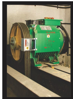
MRL / Gearless Machine
