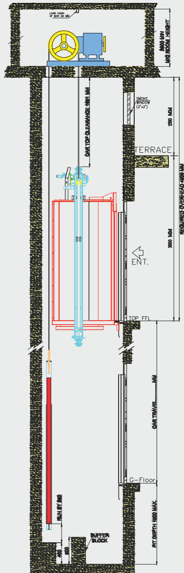
MACHINE ROOM LIFTS SECTION A-A
