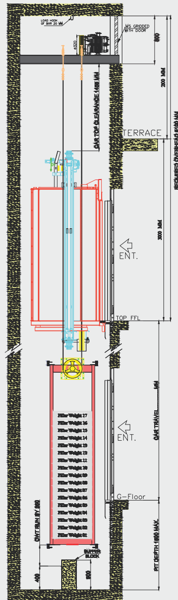
MACHINE ROOMLESS LIFTS SECTION A-A
