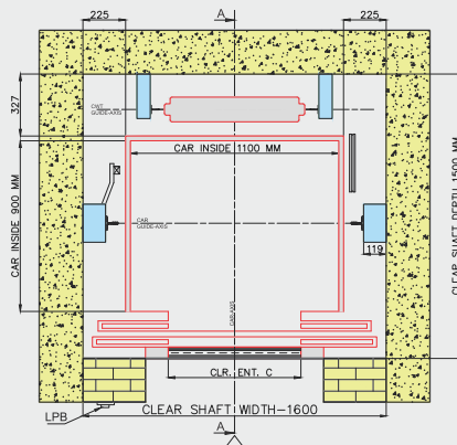
LIFT SHAFT PLAN (MR) MACHINE ROOM
