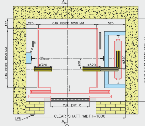
LIFT SHAFT PLAN (MRL) MACHINE ROOM LESS - BOTTOM PULLEY
