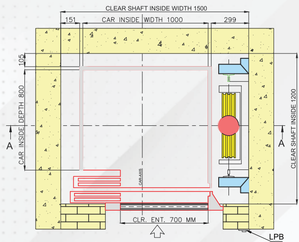
LIFT SHAFT PLAN HYDRAULIC RH-MECHANISM
