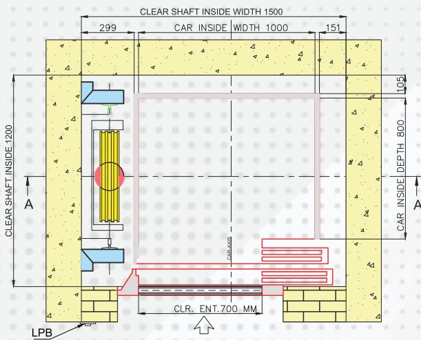
LIFT SHAFT PLAN HYDRAULIC LH-MECHANISM
