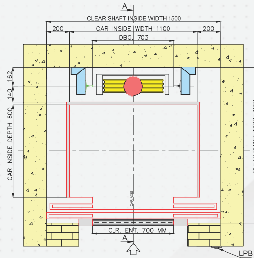
LIFT SHAFT PLAN HYDRAULIC BACK-MECHANISM
